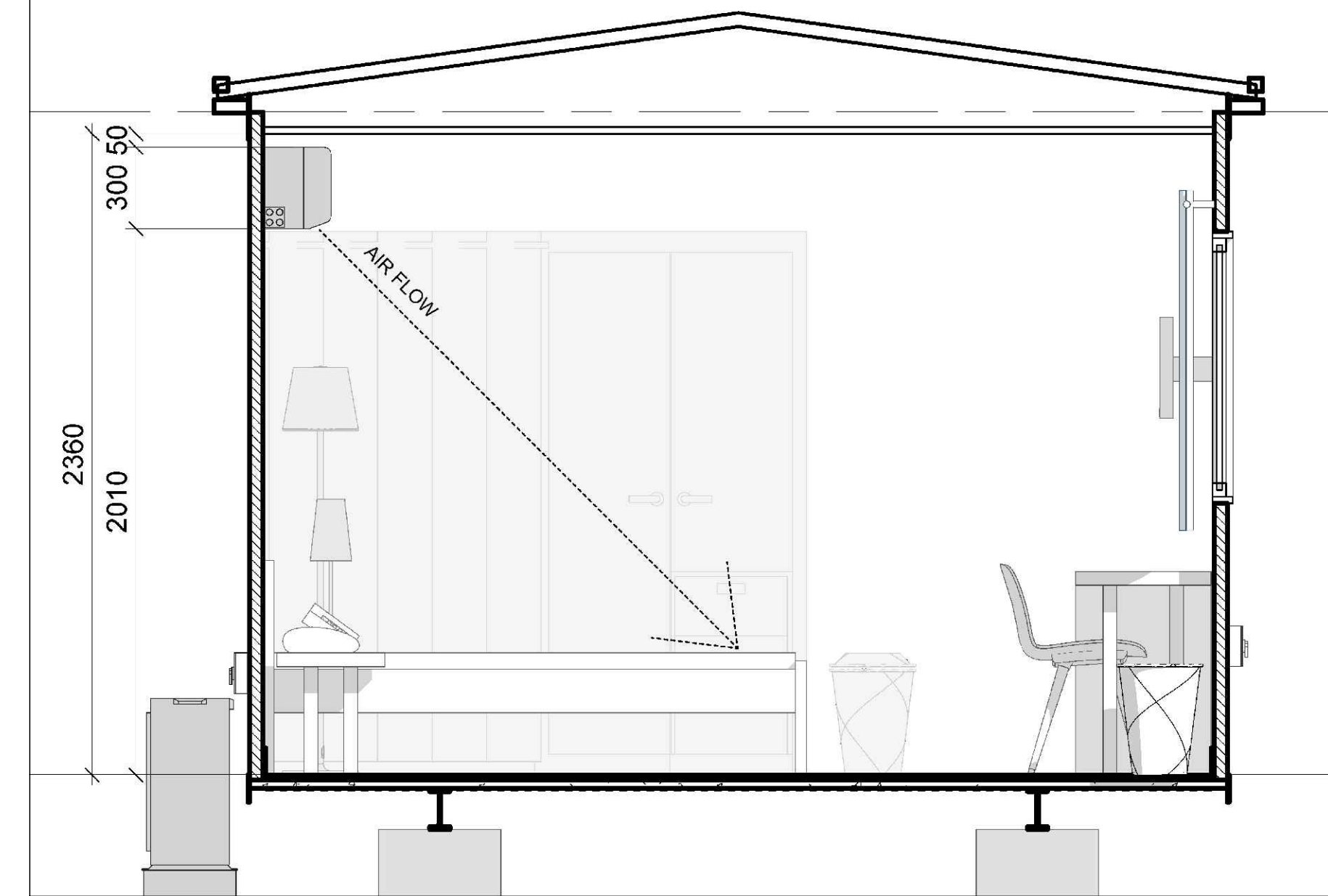
SINGLE UNIT SECTION-01
